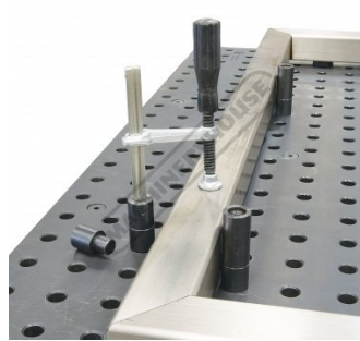
Shown Screwed into Optional Adaptor
