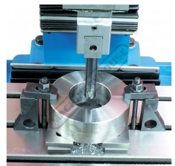
Shown Slotting Front View
