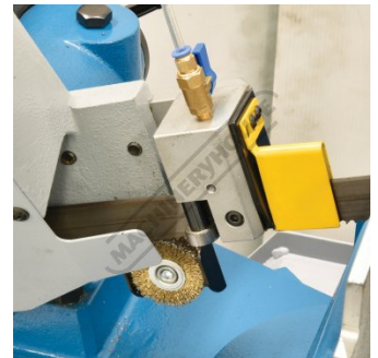
Ball Bearing Blade Guides And Cleaning Brush
