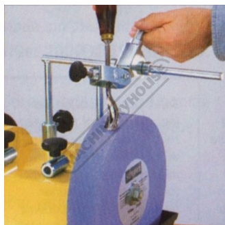
Jig 25 for retaining clamps and tubes
