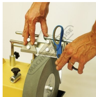
Jig 160
