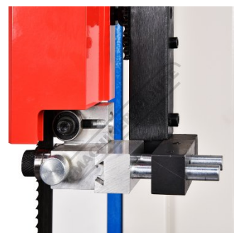
Adjustable Ball Bearing Blade Guides
