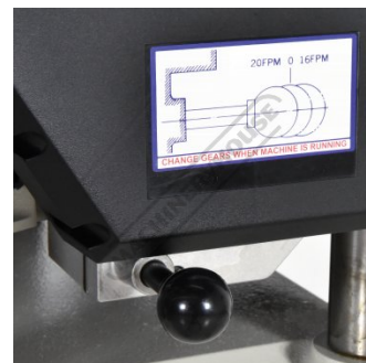
2 Speed Feed Gearbox
