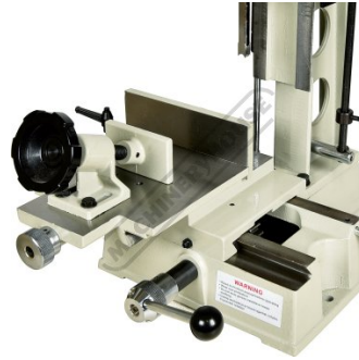
Dovetail Slideways on Work Table
