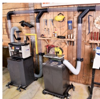
Shown Set Up with Optional Machines and Accessories 4
