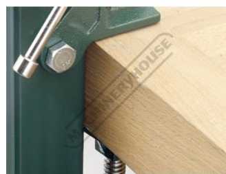
Secure Clamping
