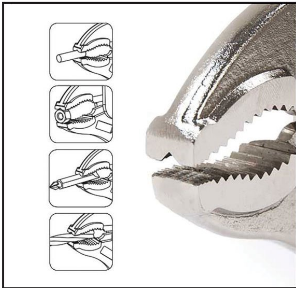
V-Groove on top jaw for holding small parts.
