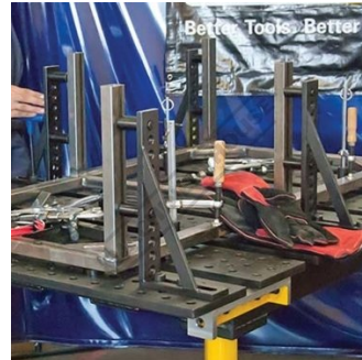
Handy and Quick to Set Up these stops can be used to Locate Stop or Position Workpieces
