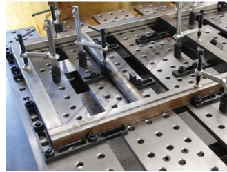
Can be Used to Locate and Set Up Stock at Right Angles
