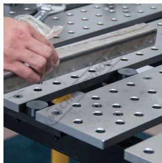
Fill any of the 40mm slots in the tabletop whenever stock or a clamp needs to be placed directly over a slot
