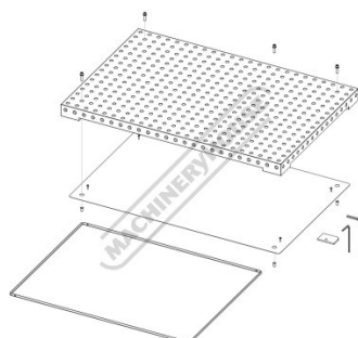
Assembly Drawing
