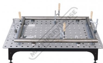
Shown with Optional Modular Fixturing Components for Round Tube 2
