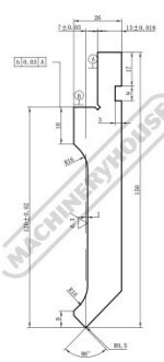
86 Degree Top Punch
