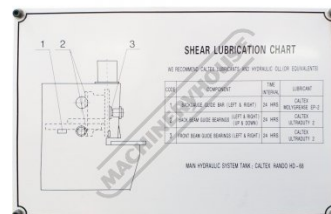
Machine Lubrication Chart
