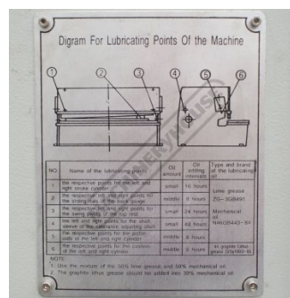
Lubrication chart
