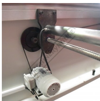
Motorised Backgauge
