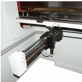
Fastfold 202 Control with Ballscrew Backgauge
