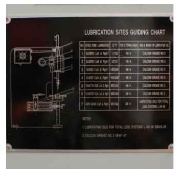
Lubrication Chart
