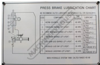
Lubrication Chart
