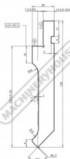
Segmented Top Punch
