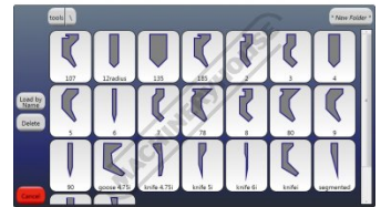
Top Punch Library
