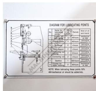
Lubrication Chart
