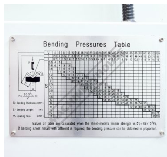
Tonnage Calculation Chart
