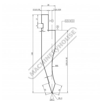
Segmented Top Punch
