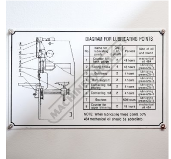
Lubrication Chart
