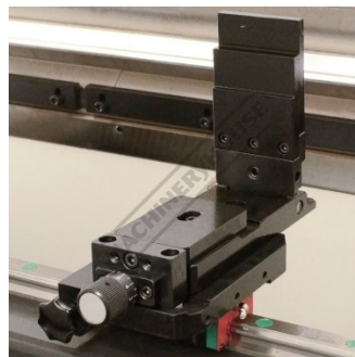
Flip up Backstop with Micro Adjustment
