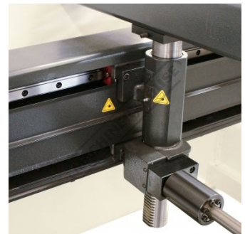
Ball Screw Backgauge with Linear Guideways
