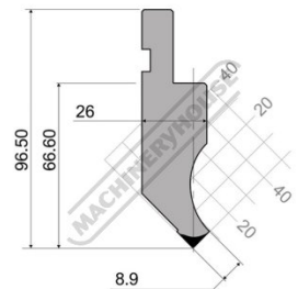
Top Tooling
