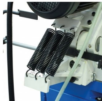
Head Return Springs
