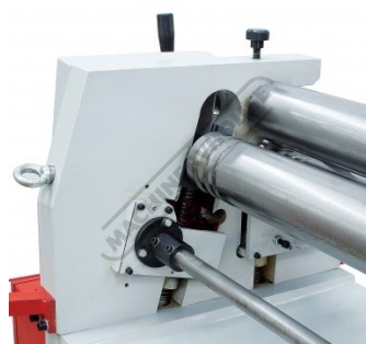
Motorised Up and Down Rear Curving Roller Left Side
