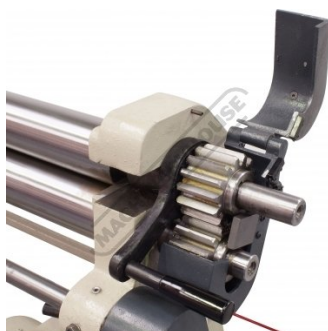
Quick Release Top Roller Handle
