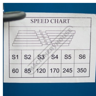
Speed Chart
