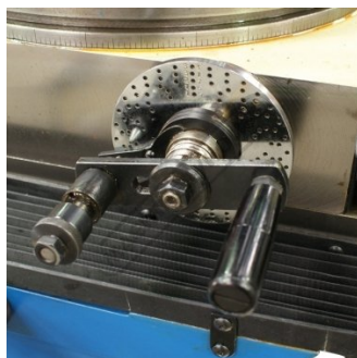
Dividing Plates
