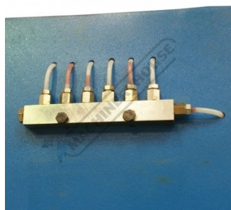
Muti Point Lubrication Block
