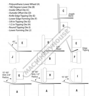
Examples of Metal Contours with Die Combinations
