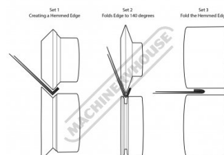
Forming A Hemmed Edges
