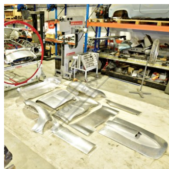
All These Car Parts Made on Power Hammer
