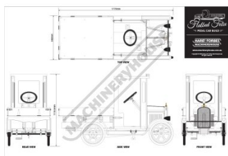
Dimesions of Finished Pedal Car
