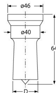
Punches 32, 38, 40
