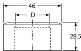
Dies 11.7 ~ 31.2
