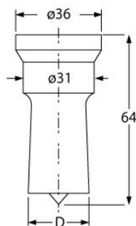
Punches 11, 13, 19, 24, 25, 28, 30
