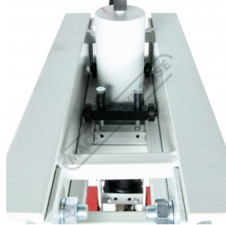
Ram Top With Breasting Slide
