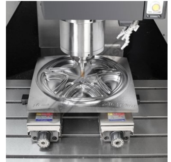
DPM650II Milling
