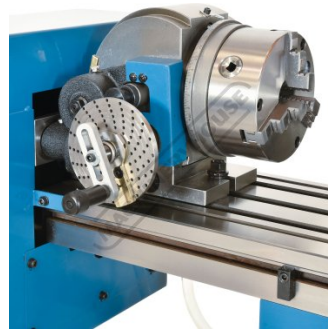
Universal Dividing Head
