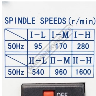
Spindle Speeds Chart
