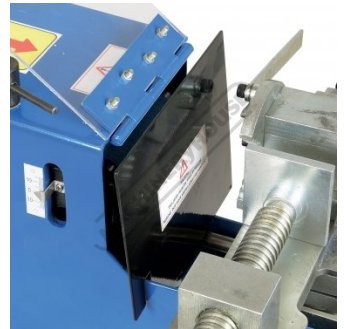
Safety Guard Inserted When Using End Sanding Station
