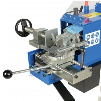
Compound Swivel Vice Right View
