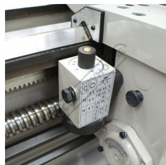
Thread Chasing Dial
