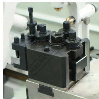
Quick Change Toolpost Rear View
