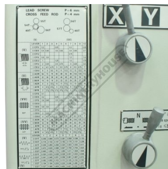
Feed Chart
