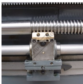
Auto engaging saddle support bearing
