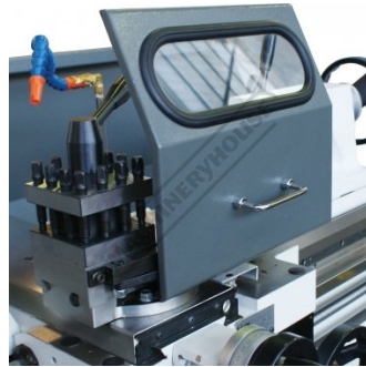
Sliding toolpost guard deflects swarf into tray-Open
