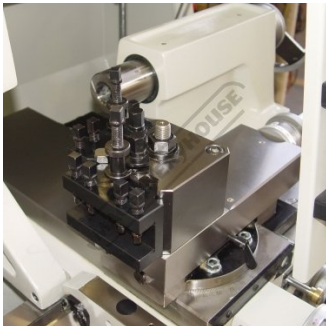
Quick change toolpost with additional holders
