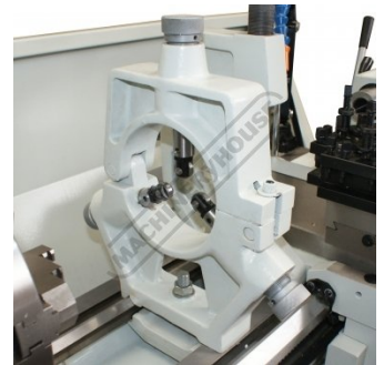
Fixed & travelling steadies with roller bearings
